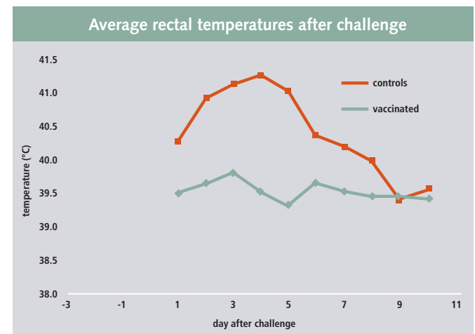
Figure 5: Average temperatures of calves after E. coli challenge
