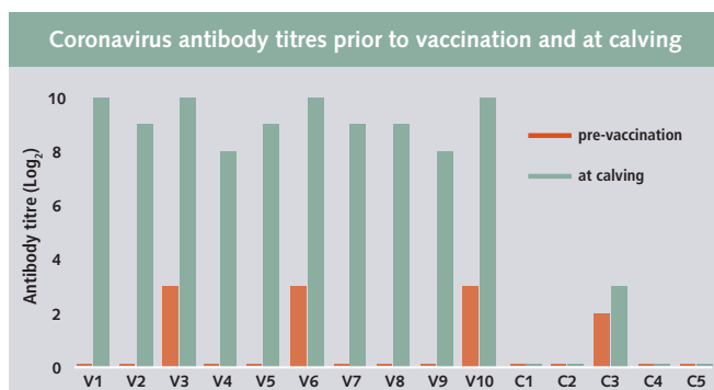
Figure 6: Coronavirus antibody titres in dams
