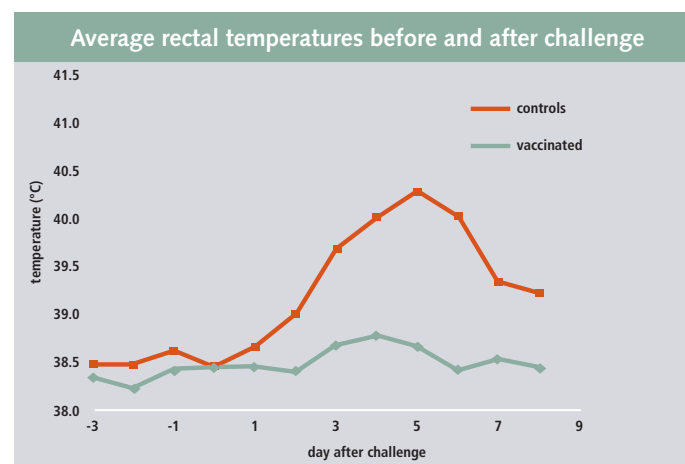
Figure 2: Average temperatures of calves after rotavirus challenge.
