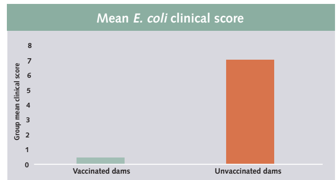
Figure 4: Mean clinical score in calves challenged with enteropathogenic E. coli
