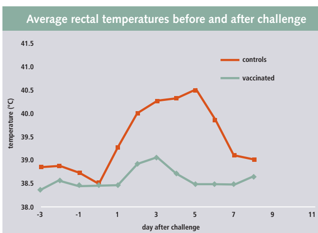
Figure 7: Average temperature of calves after bovine coronavirus challenge
