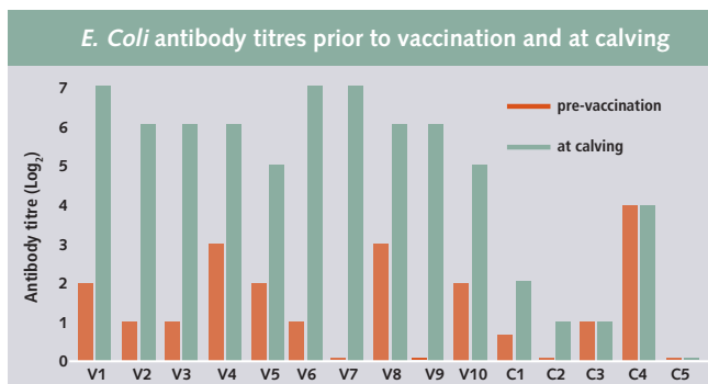
Figure 3: E. coli antibody titres in dams
