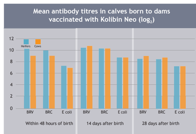
Figure 2. Mean antibody titre to each of the enteropathogens in Kolibin Neo in calves born to heifers and cows at within 48 hours of their birth and at 14 and 28 days of age.
