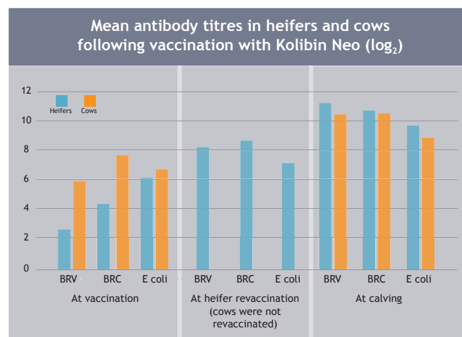
Figure 1. Mean antibody titre to each of the enteropathogens in Kolibin Neo in heifers and cows at vaccination, at revaccination and at calving.
